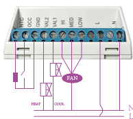
Connection 2: 4-pipe ON/OFF +3 speed fan
