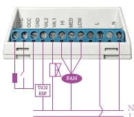
Connection 4: 2-pipe ON/OFF +TIO2/ESP
