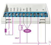
Connection 6: Underfloor Heating
