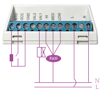
Connection 1: 2-pipe ON/OFF +3 speed fan
