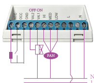
Connection 5: 2-pipe ON/OFF +3 wire valve
