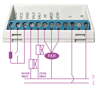
Connection 3: 2-pipe ON/OFF +floor heating
