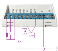
Connection 7: Water Source Heat Pump
